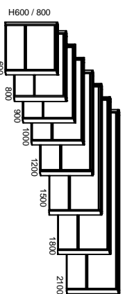
Suspended Screens with hanging rail & divider rail
