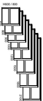
Suspended Screens with function wall top
