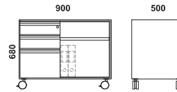
Combo Unit -BBF/Open
