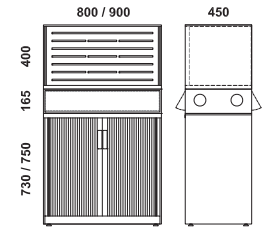
Tambour Combo Unit with Cable Box
